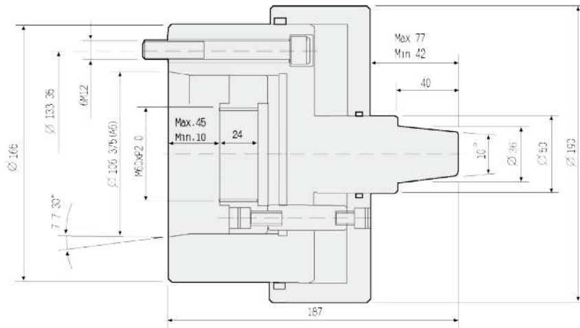
Product schematic
